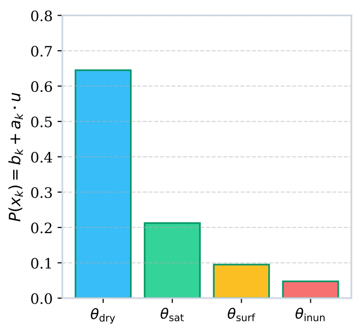
3. Projected Probability P(x_k)
