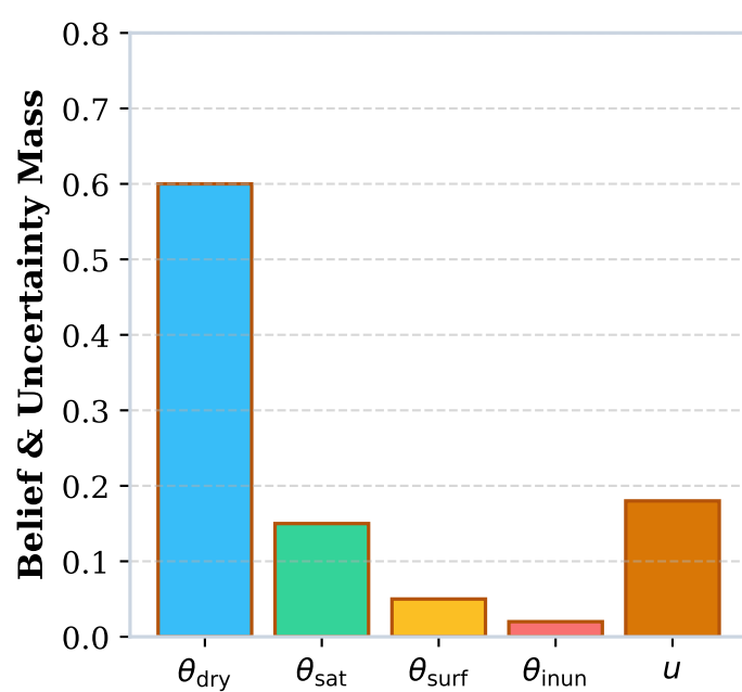
2. Opinion Tuple (b, u, a)
