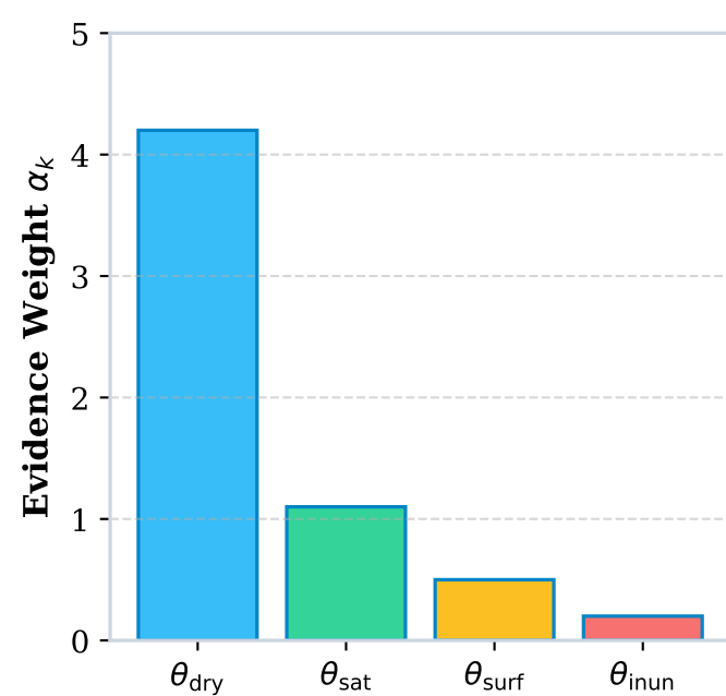
1. Dirichlet Evidence \alpha
